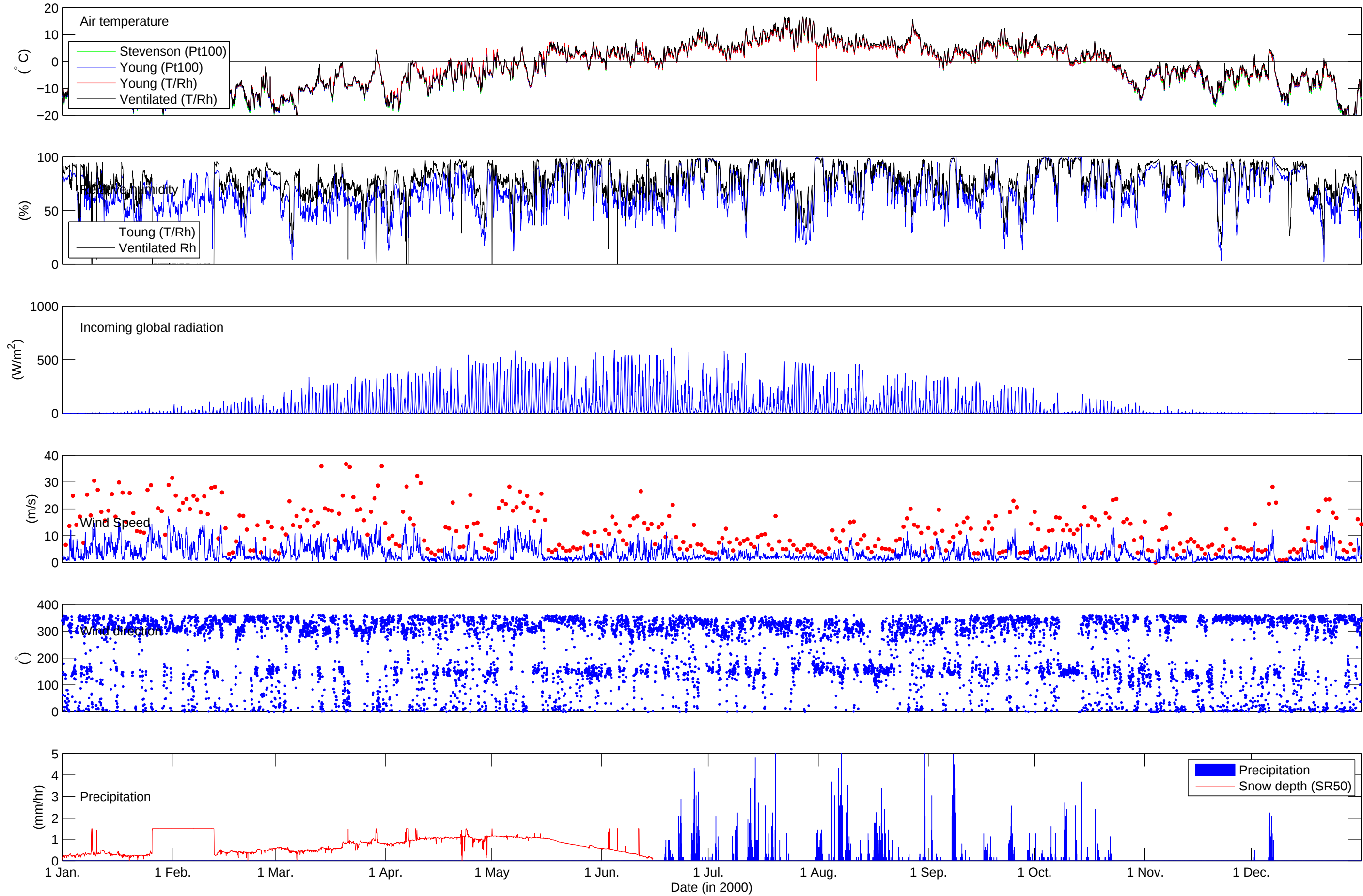
Tarfala Research Station meteorological data for 2000
